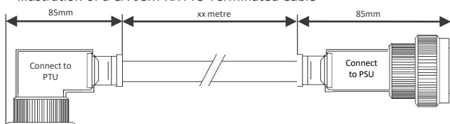
Illustration of a CA-JCM-XX Pre-Terminated Cable
