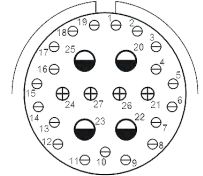
Connector (Pre-Terminated)
